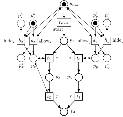
(c) Configurable interface N_\beta^{CI} (block by default)
