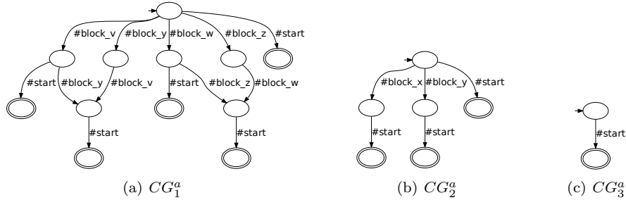
Figure 10: The configuration guidelines (allow by default) for N_1 (a), N_2 (b) and N_3 (c). Hiding actions are not depicted.
