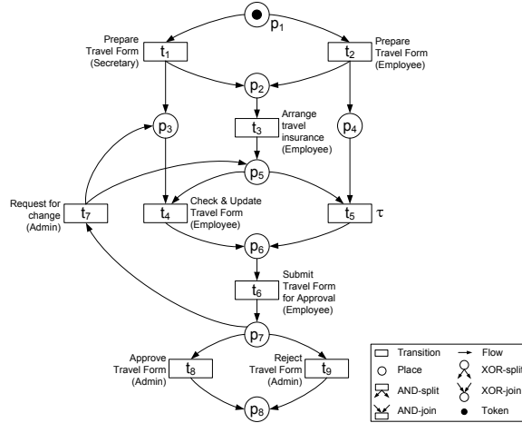
Figure 5: The open net for travel request approval ( \Omega = \{[p_8]\} ).
