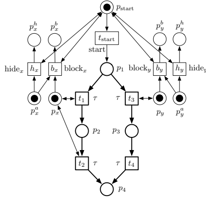
(b) Configurable interface N_\alpha^{CI} (allow by default)
