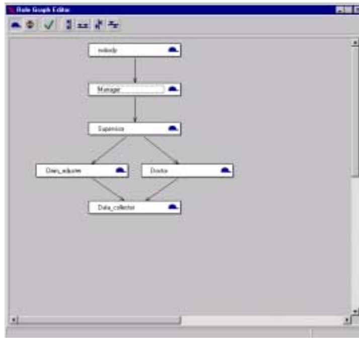
Figure 10: Role graph editor of Studio showing the six roles involved.
