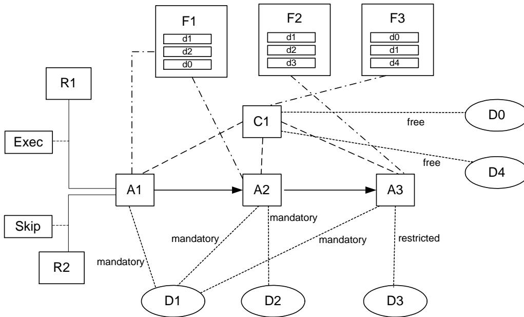
Figure 2: Abstract example introducing the schema level of the case handling meta model.
