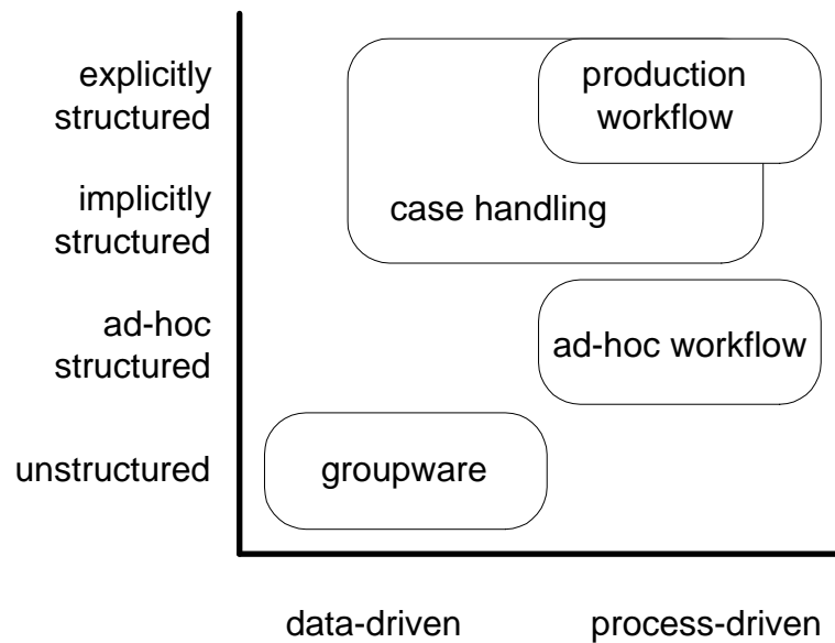
Figure 14: Positioning case handling.
