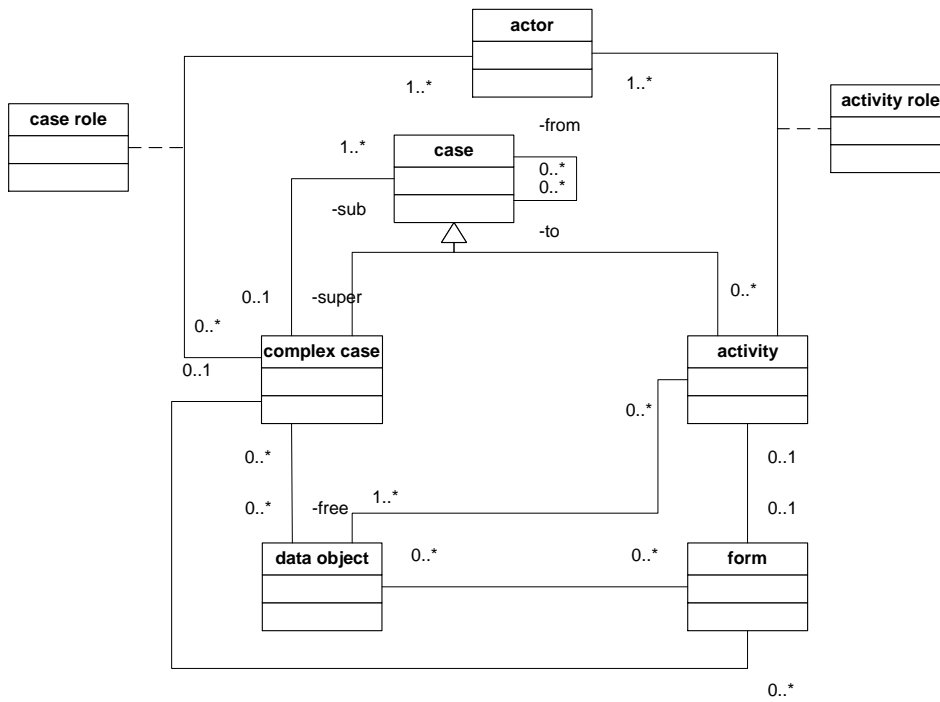
Figure 3: Case handling meta model, instance level.
