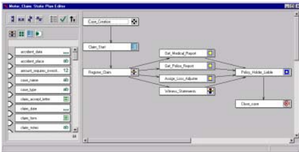
Figure 6: Complex case definition MotorClaim .
