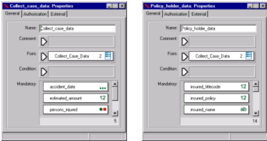
Figure 9: Properties of activities, including specification of mandatory data objects.
