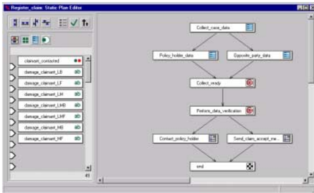
Figure 7: Complex case definition Register.Claim .
