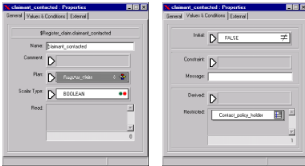
Figure 8: Attributes of the data object definition claimant_contacted .
