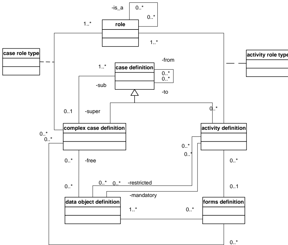
Figure 1: Case handling meta model, schema level.
