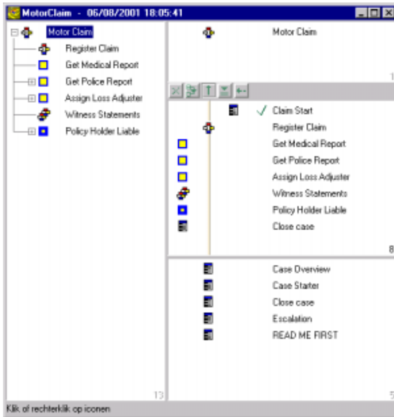
Figure 12: The FLOWer Case Guide.
